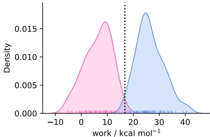
complex ( N = 83 )
