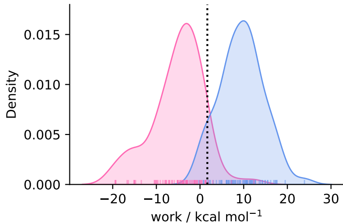
complex ( N = 76 )
