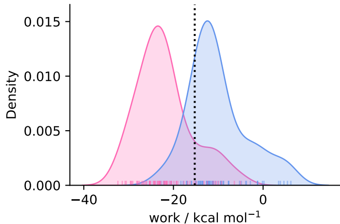
complex ( N = 67 )
