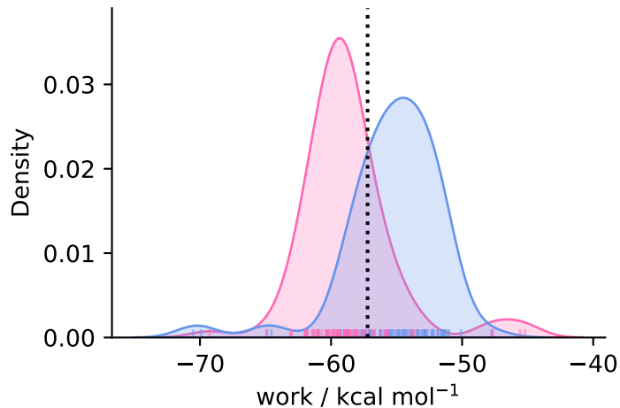
complex ( N = 87 )
