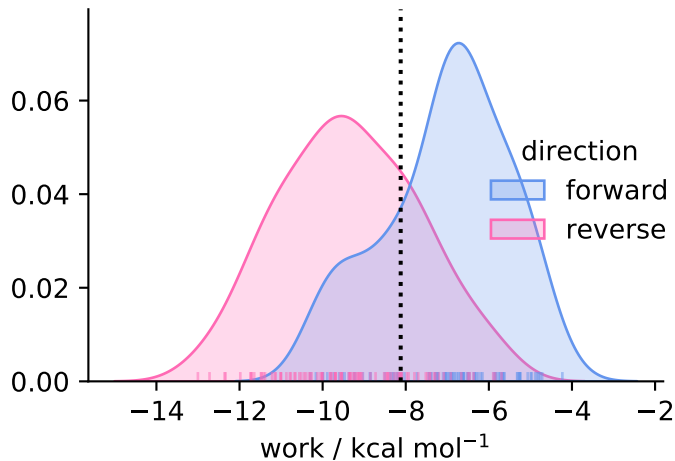
solvent ( N = 96 )
