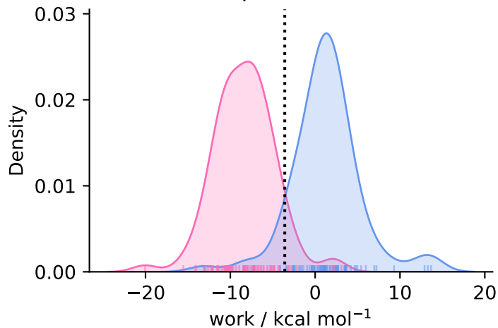
complex ( N = 81 )
