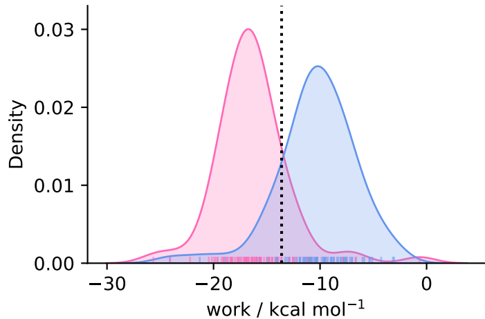
complex ( N = 73 )
