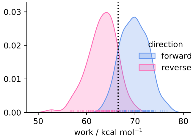
solvent ( N = 100 )
