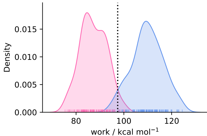
complex ( N = 118 )
