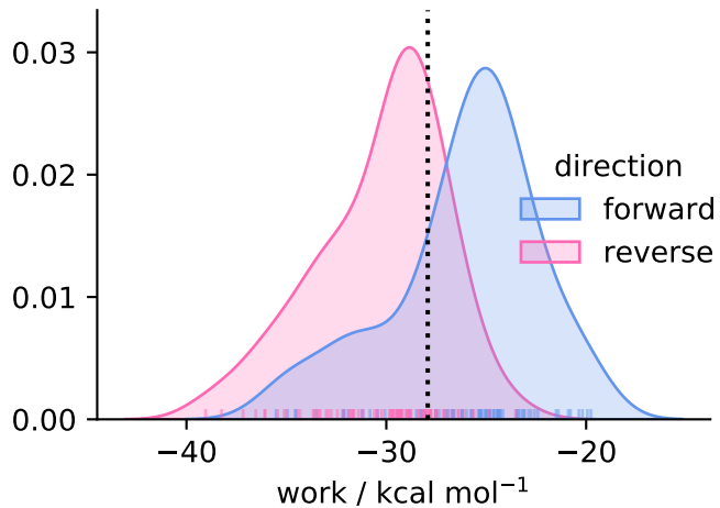
solvent ( N = 79 )
