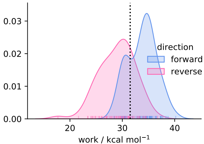
solvent ( N = 77 )
