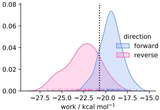
solvent ( N = 79 )
