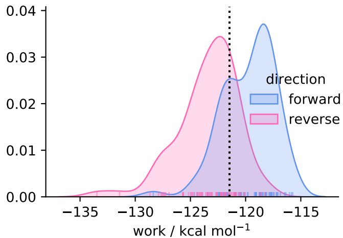
solvent ( N = 78 )
