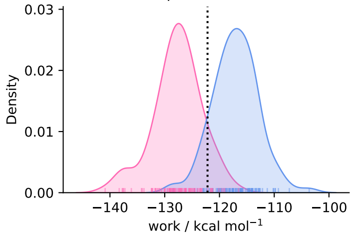
complex ( N = 103 )
