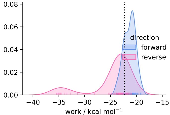
solvent ( N = 80 )
