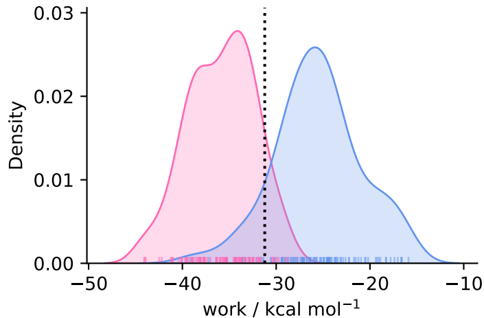
complex ( N = 101 )
