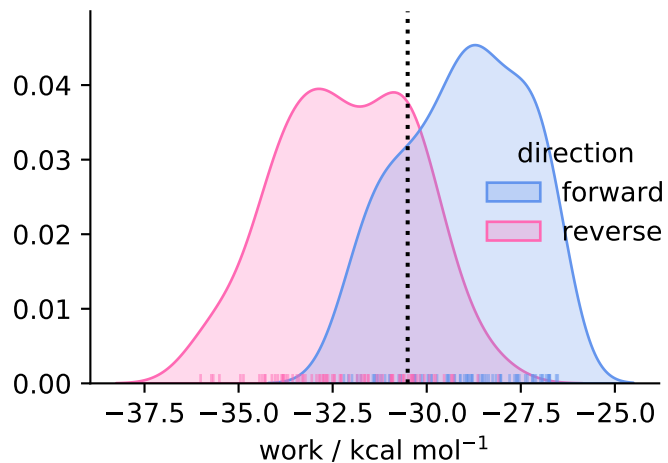
solvent ( N = 80 )
