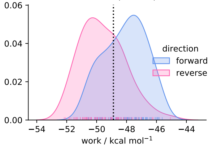
solvent ( N = 79 )
