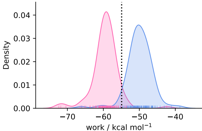
complex ( N = 101 )
