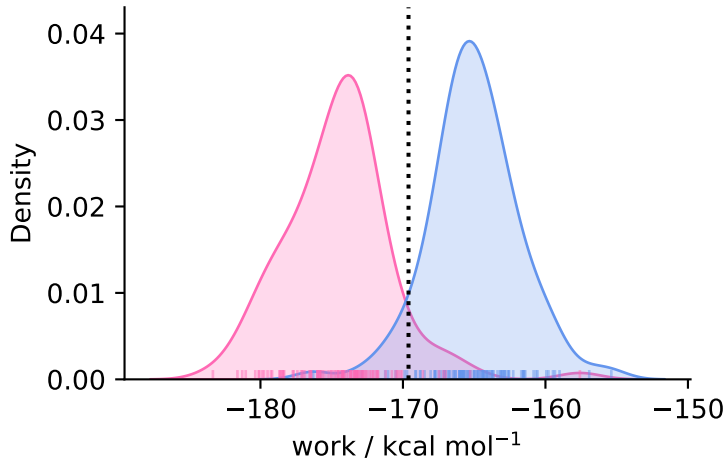
complex ( N = 104 )
