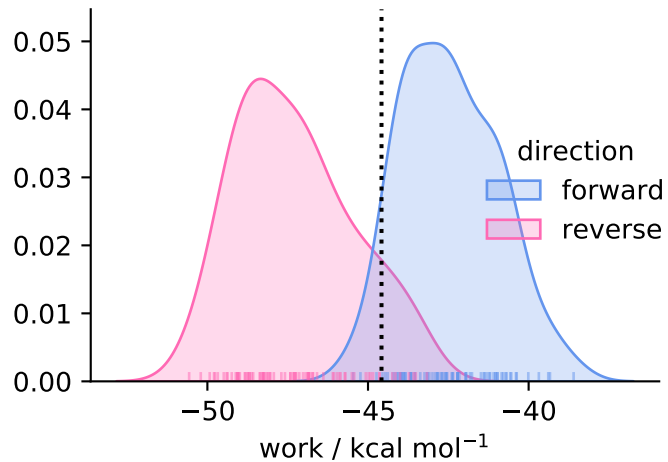
solvent ( N = 79 )
