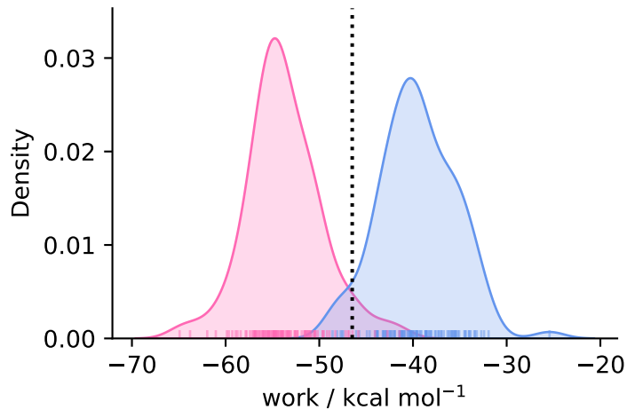
complex ( N = 103 )
