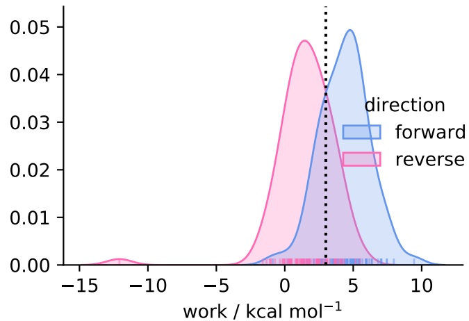
solvent ( N = 79 )
