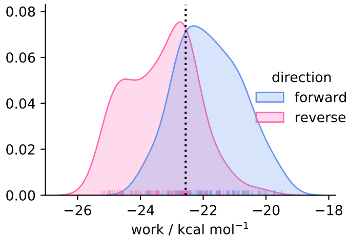
solvent ( N = 79 )
