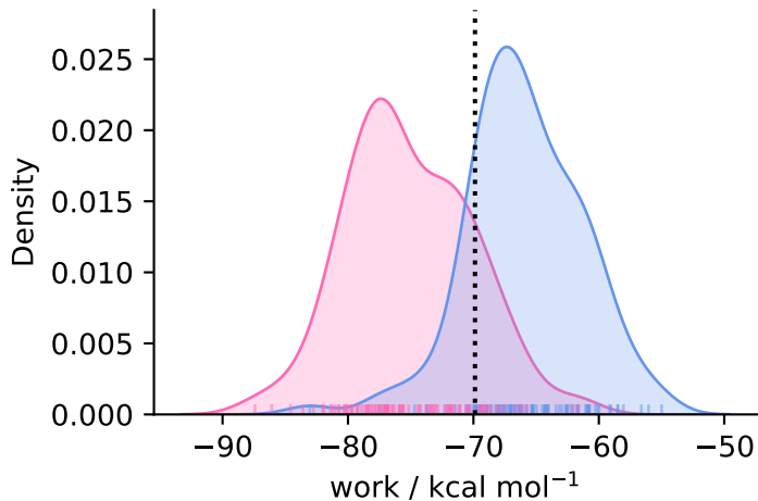
complex ( N = 105 )
