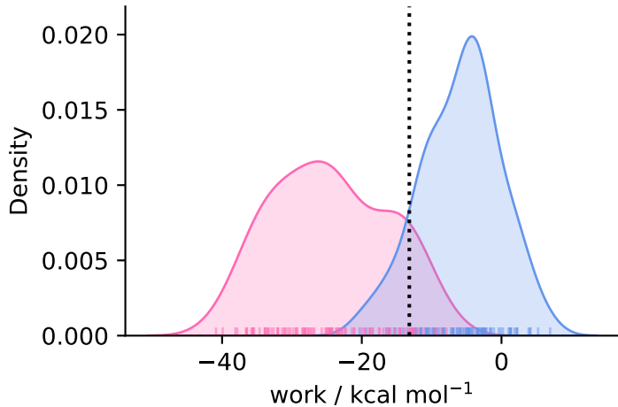
complex ( N = 104 )
