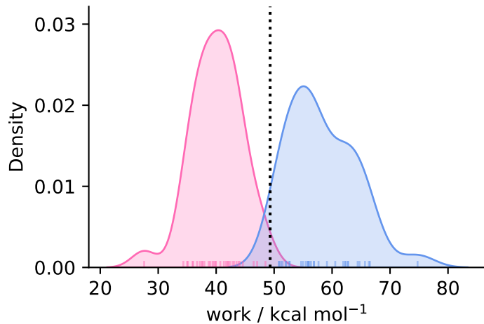
complex ( N = 32 )
