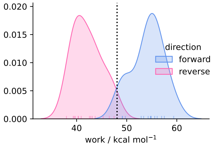
solvent ( N = 14 )
