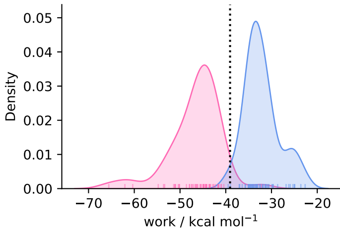
complex ( N = 54 )
