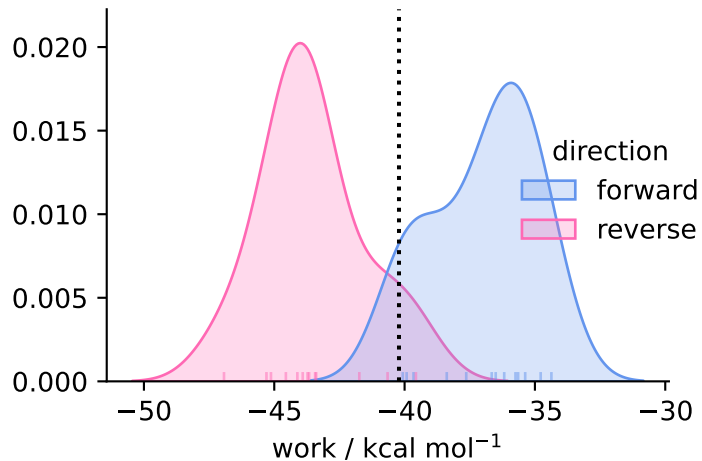
solvent ( N = 13 )
