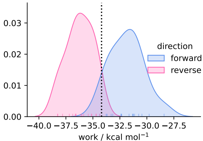
solvent ( N = 17 )
