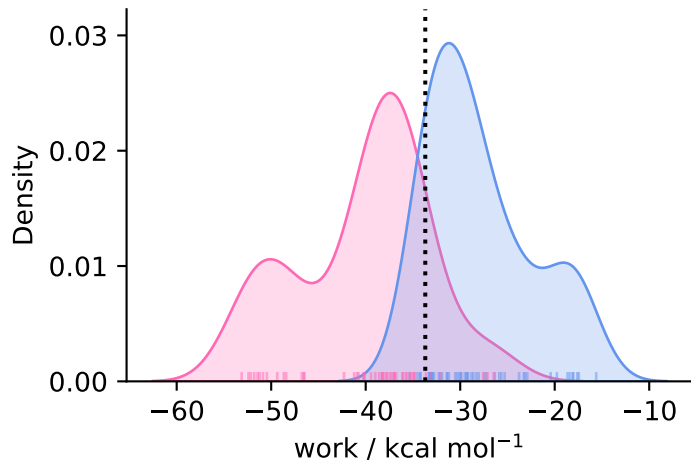
complex ( N = 51 )
