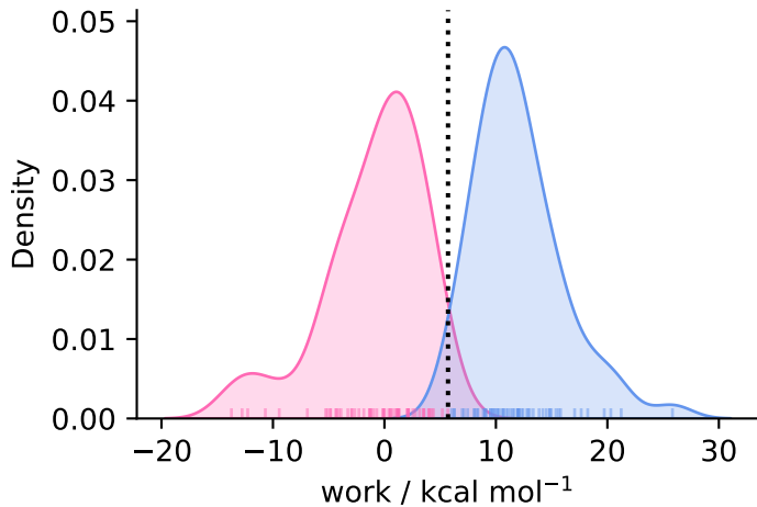
complex ( N = 59 )
