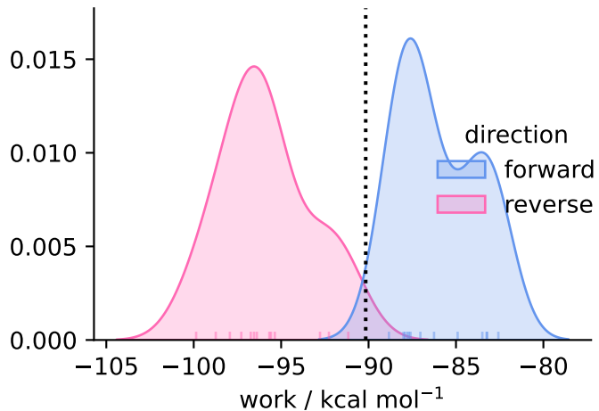
solvent ( N = 13 )
