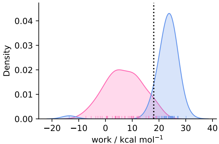
complex ( N = 46 )
