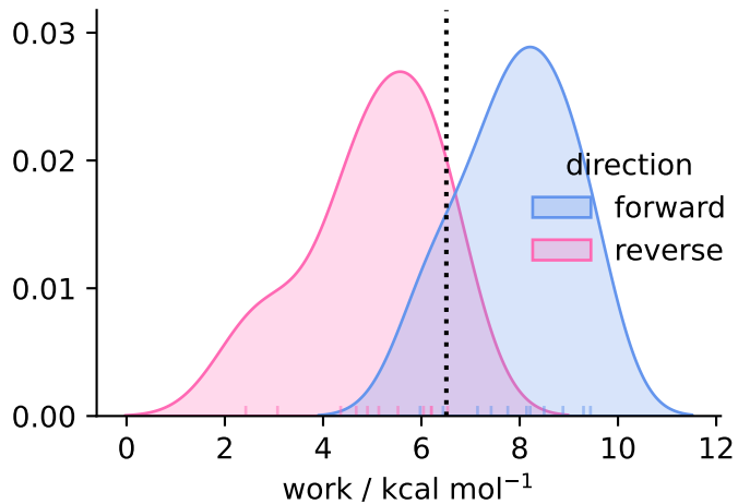
solvent ( N = 11 )
