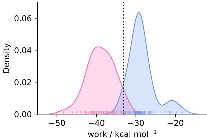
complex ( N = 57 )
