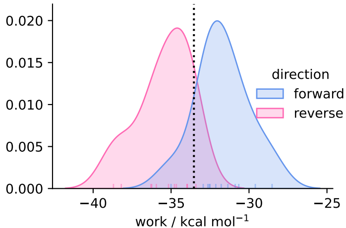
solvent ( N = 12 )
