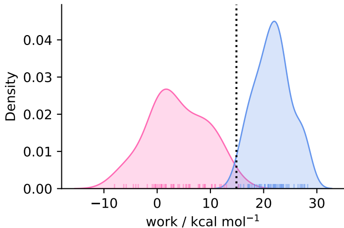
complex ( N = 51 )
