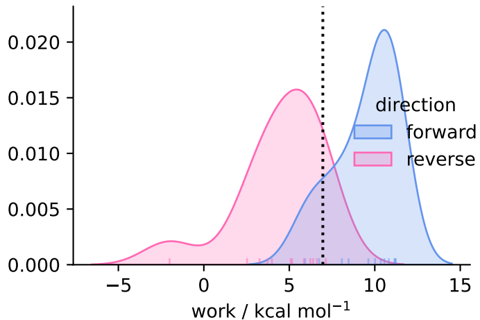
solvent ( N = 12 )
