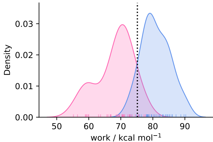
complex ( N = 41 )
