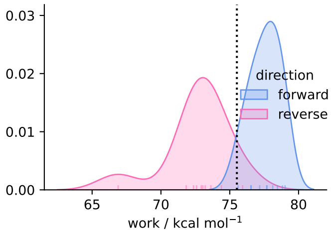
solvent ( N = 10 )
