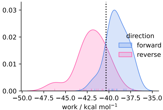
solvent ( N = 13 )
