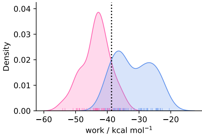
complex ( N = 50 )
