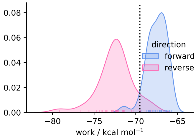
solvent ( N = 37 )
