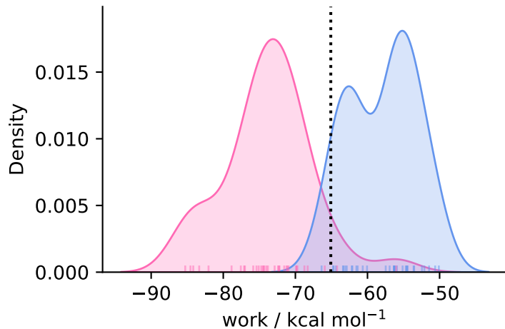
complex ( N = 34 )
