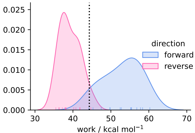
solvent ( N = 14 )
