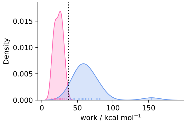
complex ( N = 23 )
