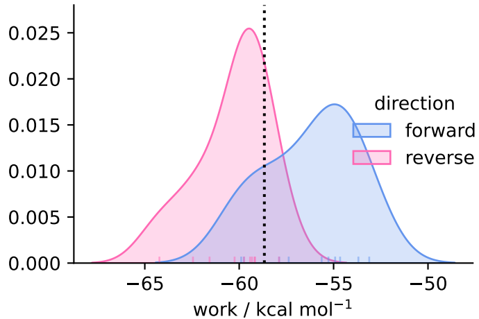
solvent ( N = 10 )
