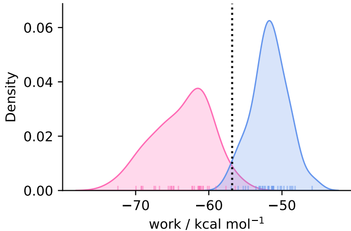
complex ( N = 32 )
