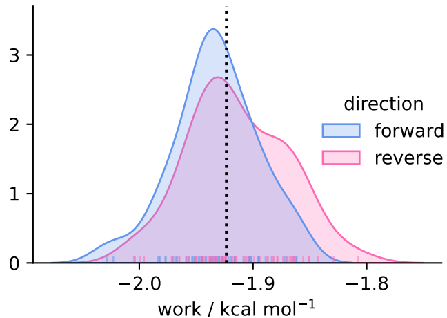
solvent ( N = 59 )
