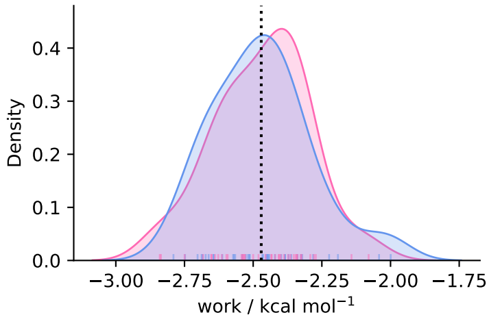
complex ( N = 39 )
