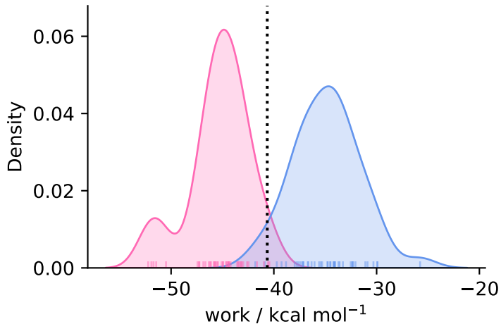
complex ( N = 42 )
