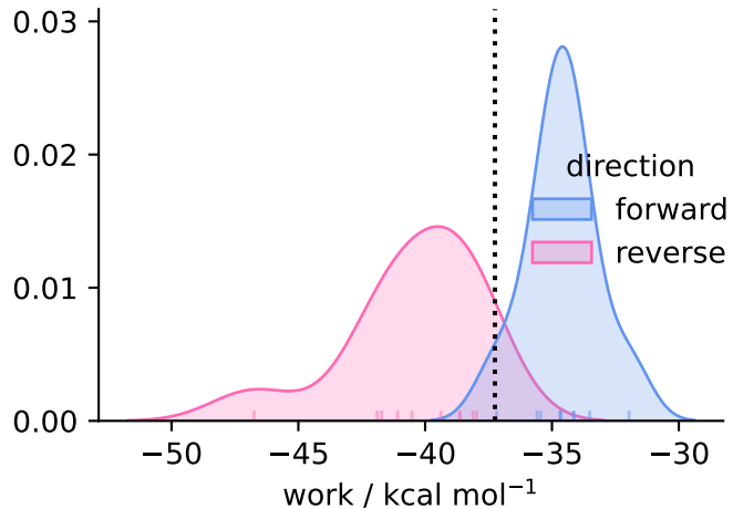
solvent ( N = 10 )
