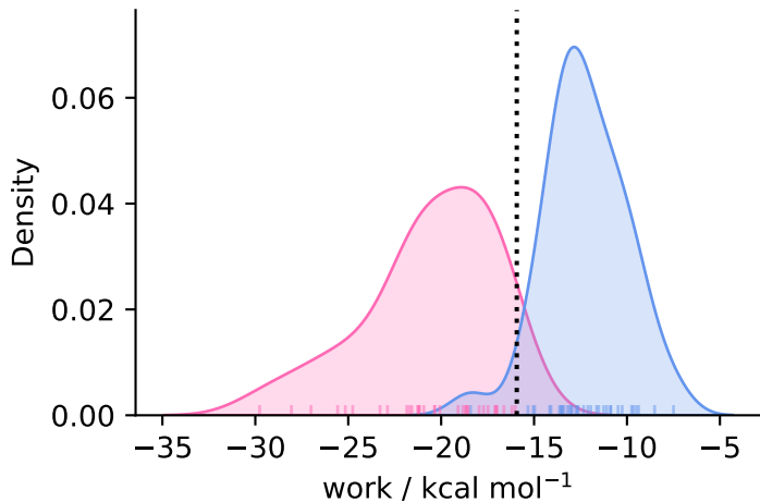
complex ( N = 35 )
