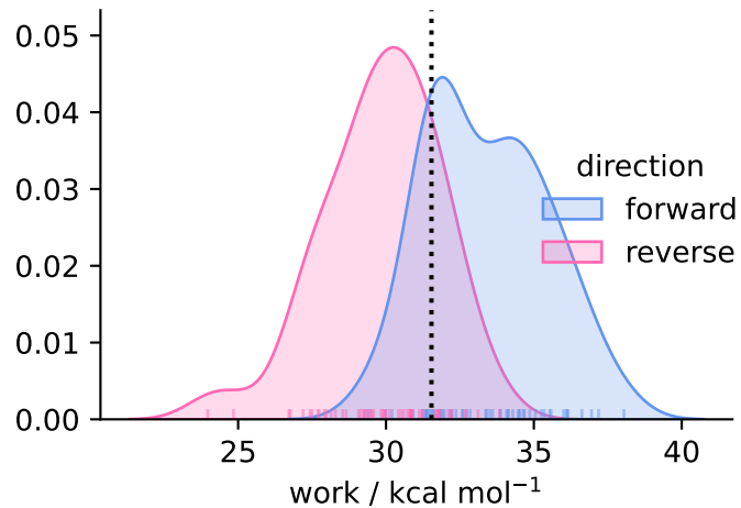
solvent ( N = 56 )
