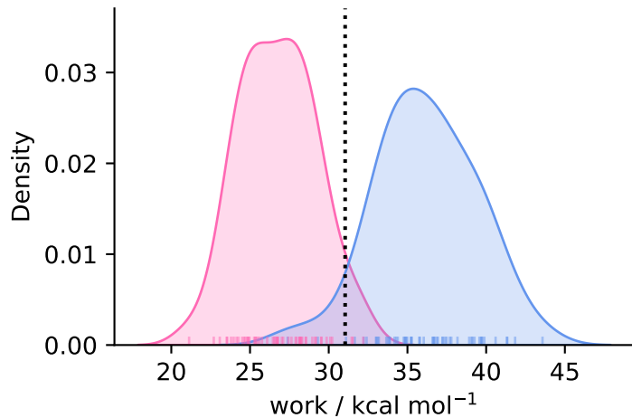
complex ( N = 55 )
