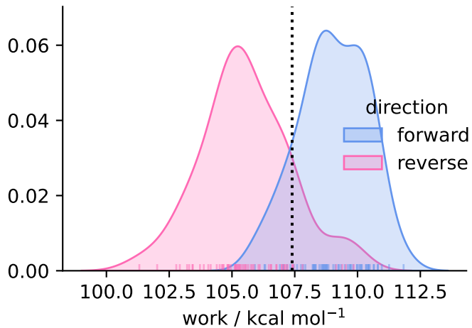
solvent ( N = 60 )
