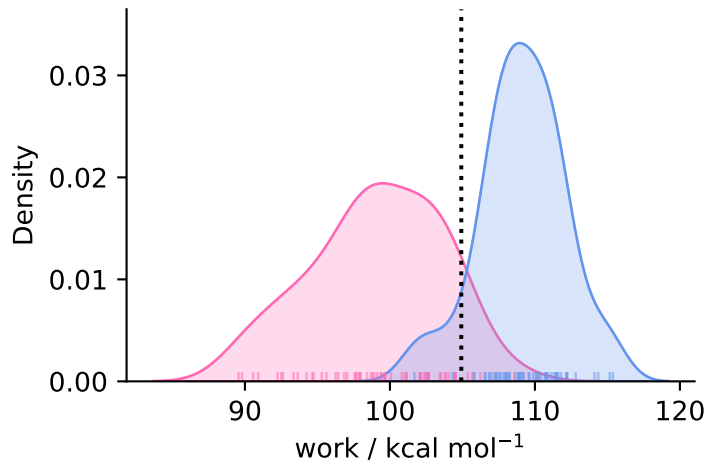
complex ( N = 59 )
