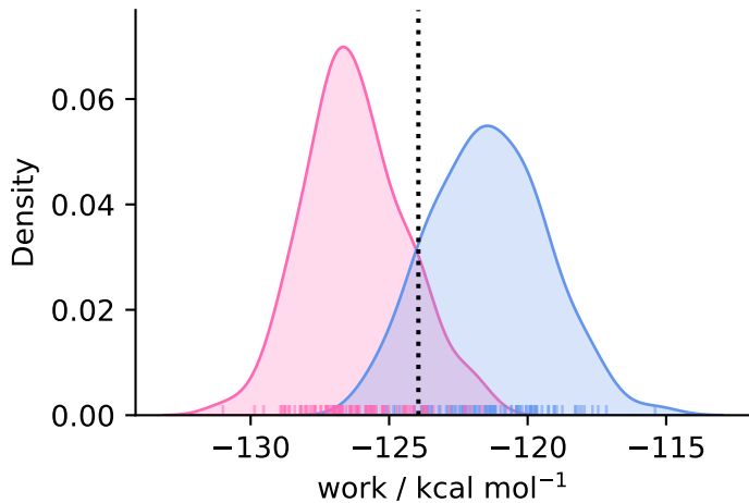
complex ( N = 100 )
