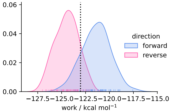
solvent ( N = 60 )
