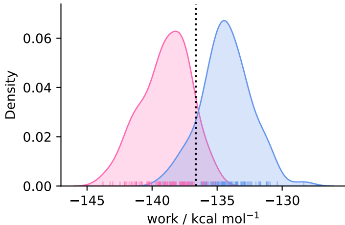
complex ( N = 100 )
