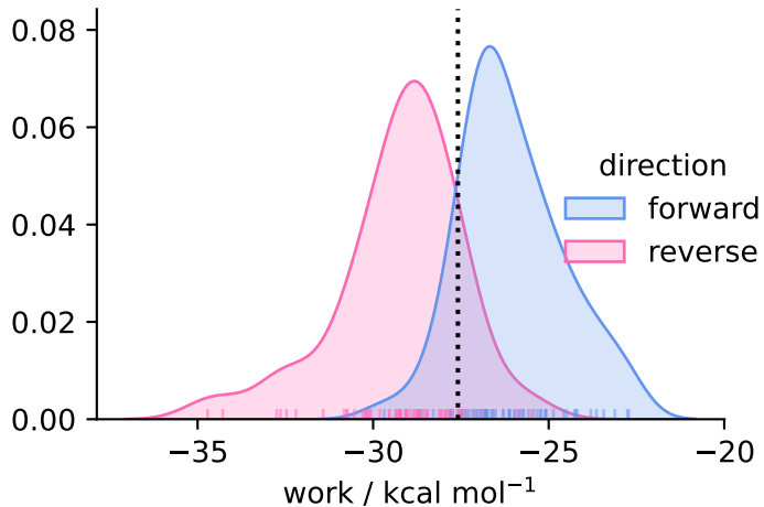
solvent ( N = 60 )
