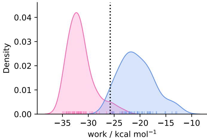
complex ( N = 52 )
