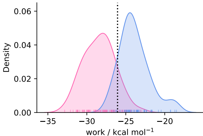
complex ( N = 67 )
