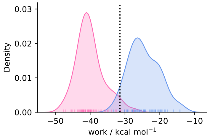
complex ( N = 60 )
