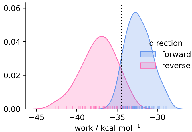
solvent ( N = 60 )
