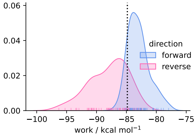
solvent ( N = 59 )
