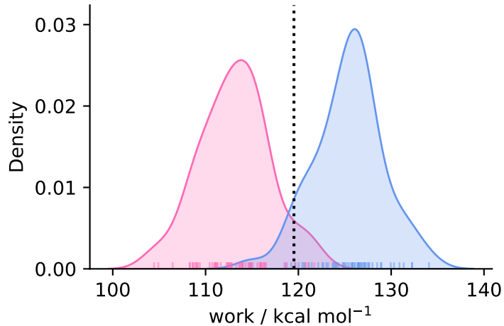
complex ( N = 59 )
