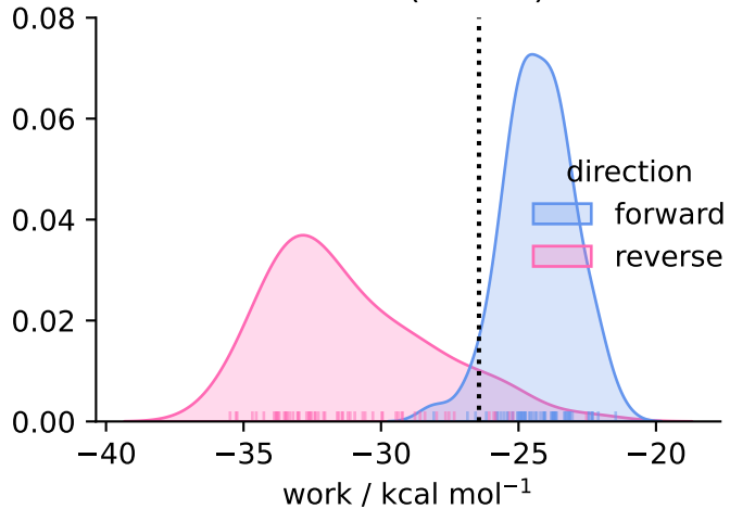
solvent ( N = 60 )
