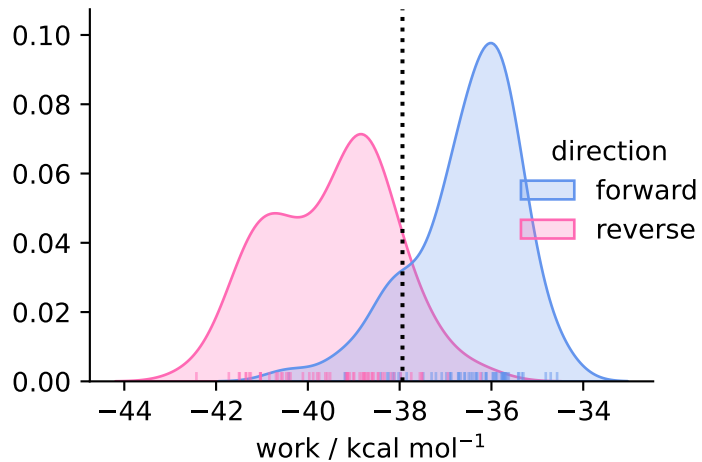
solvent ( N = 60 )
