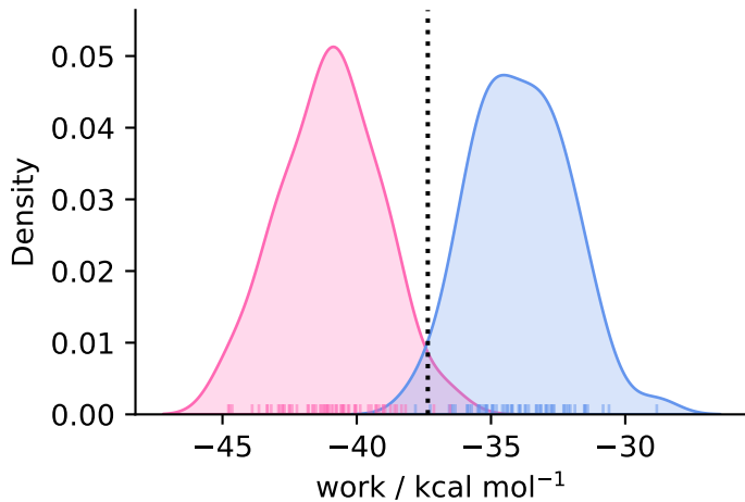
complex ( N = 60 )
